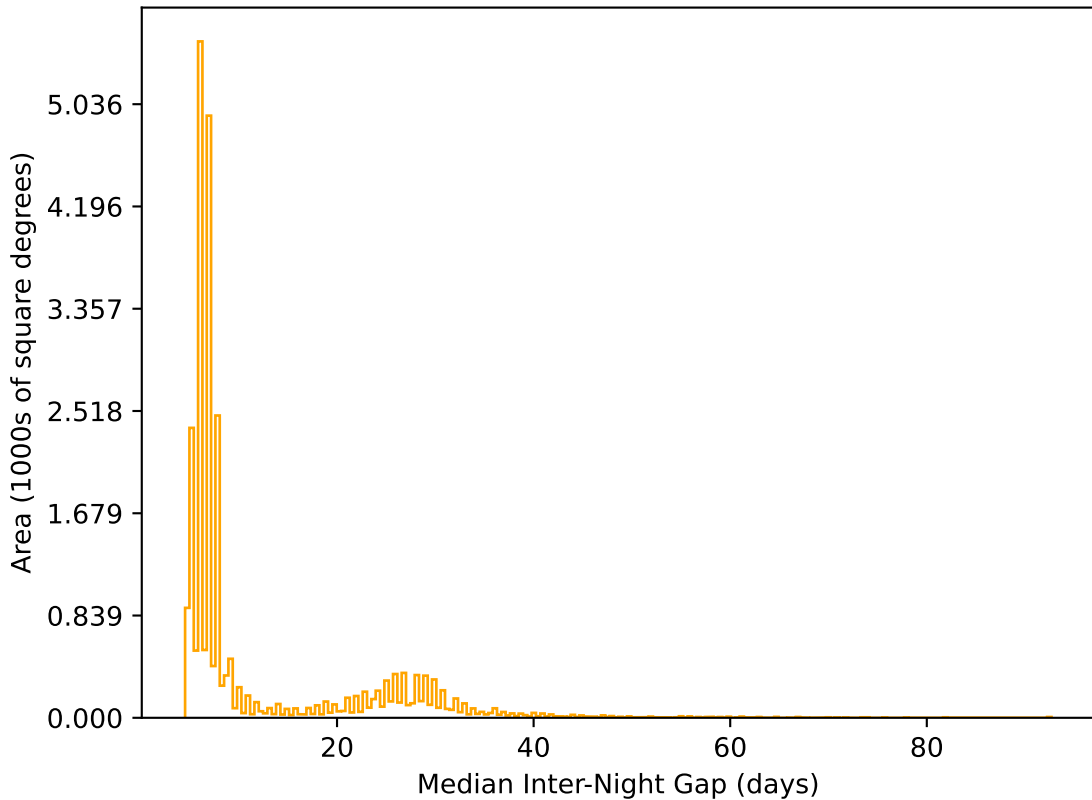
roll_pause_mjdp180_v3.4_10yrs All sky r band: Median Inter-Night Gap
