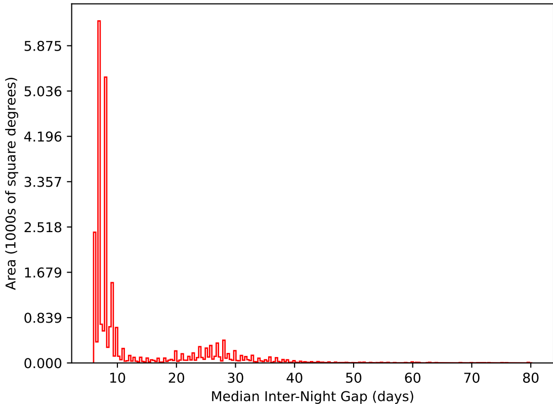
roll_pause_mjdp180_v3.4_10yrs All sky i band: Median Inter-Night Gap
