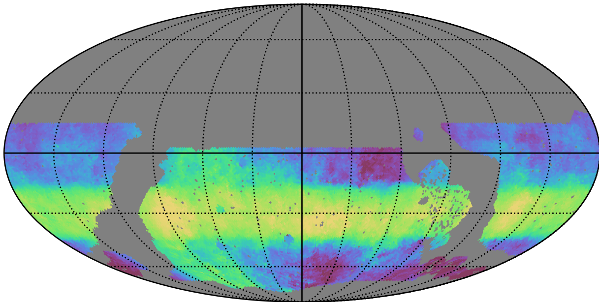
roll_pause_mjdp180_v3.4_10yrs WFD z band: Median HA
