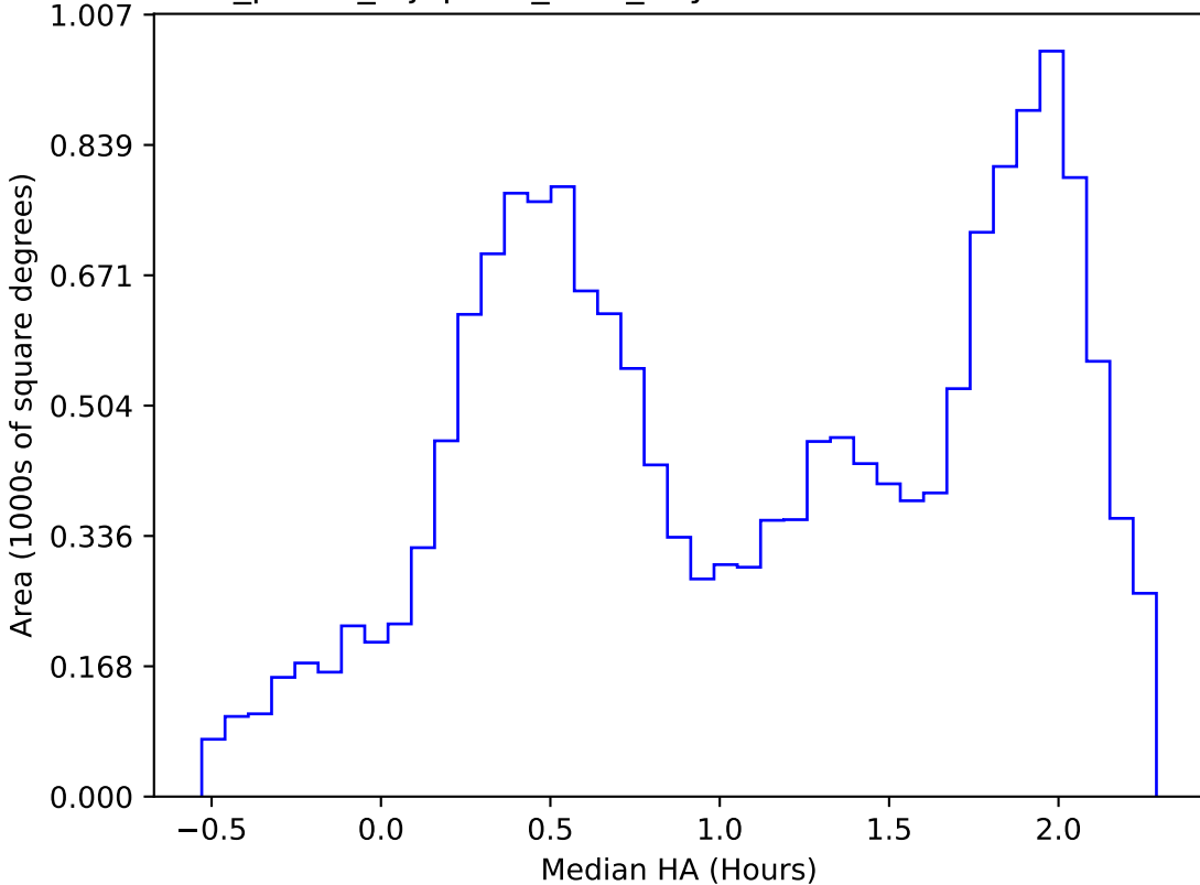
roll_pause_mjdp180_v3.4_10yrs WFD z band: Median HA
