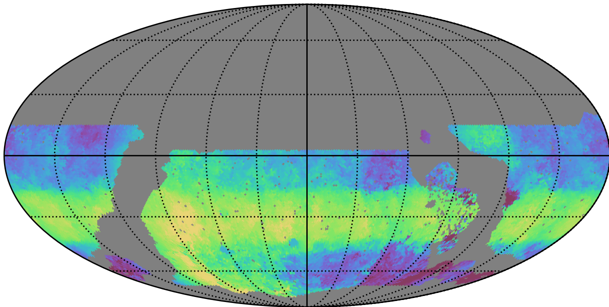
roll_pause_mjdp180_v3.4_10yrs WFD u band: Median HA
