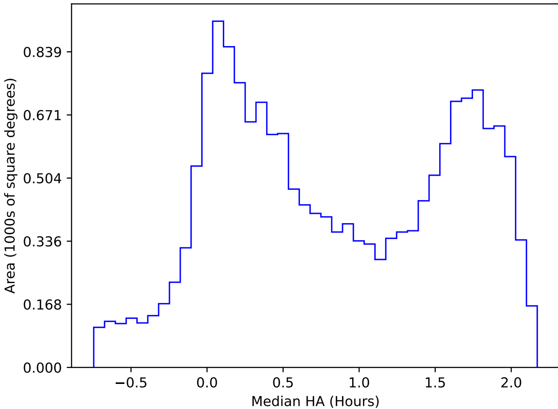
roll_pause_mjdp180_v3.4_10yrs WFD r band: Median HA
