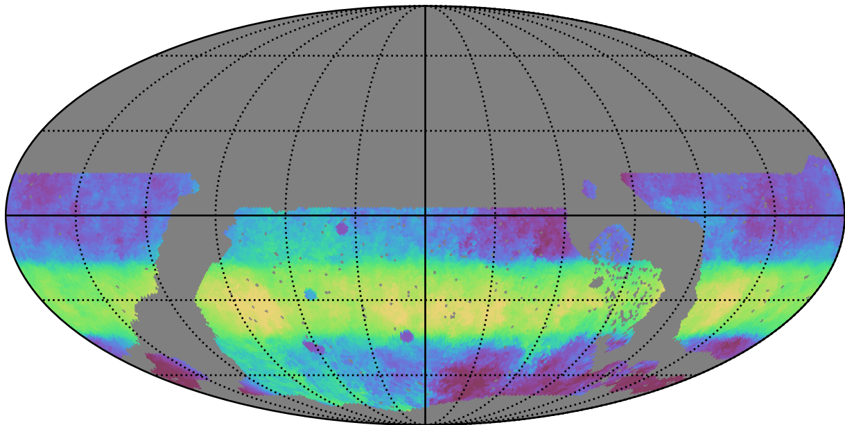
roll_pause_mjdp180_v3.4_10yrs WFD i band: Median HA
