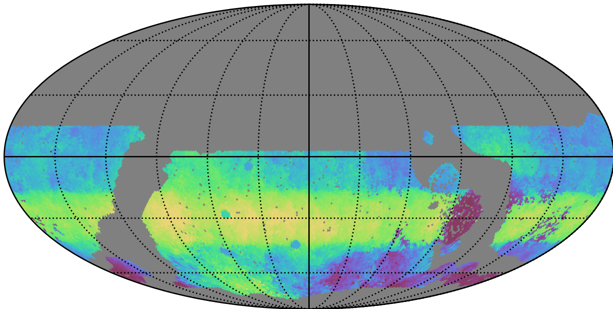
roll_pause_mjdp180_v3.4_10yrs WFD g band: Median HA
