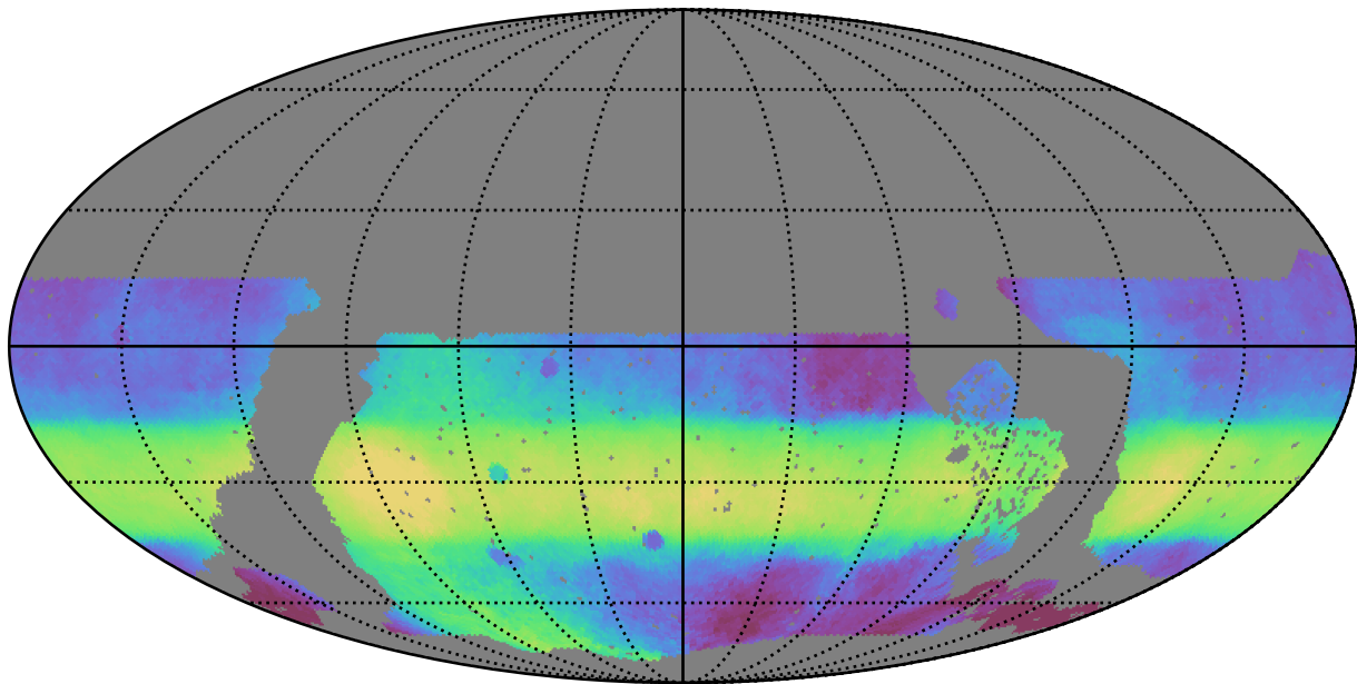
roll_pause_mjdp180_v3.4_10yrs WFD all bands: Median HA
