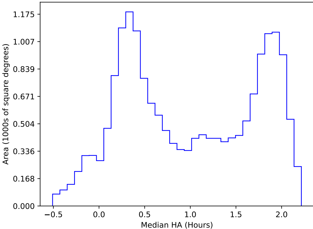
roll_pause_mjdp180_v3.4_10yrs WFD all bands: Median HA
