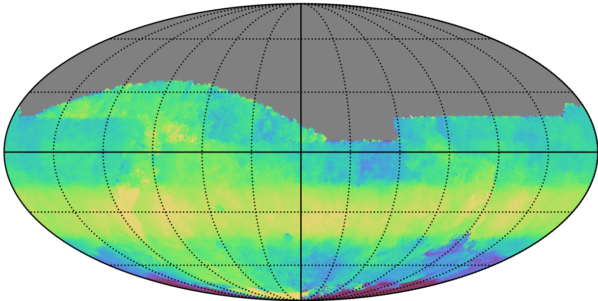
roll_pause_mjdp180_v3.4_10yrs All sky z band: Median HA
