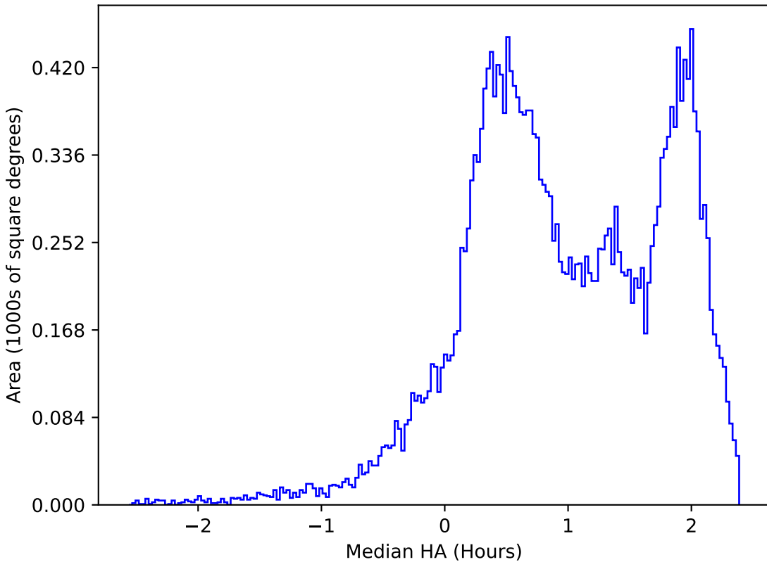
roll_pause_mjdp180_v3.4_10yrs All sky z band: Median HA
