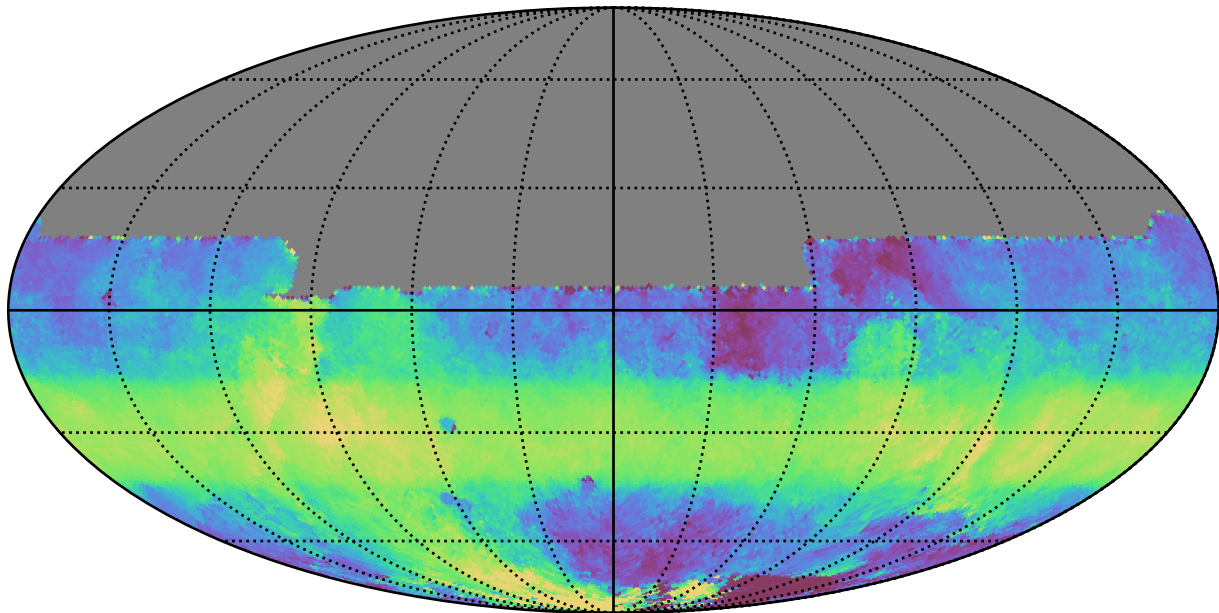
roll_pause_mjdp180_v3.4_10yrs All sky y band: Median HA
