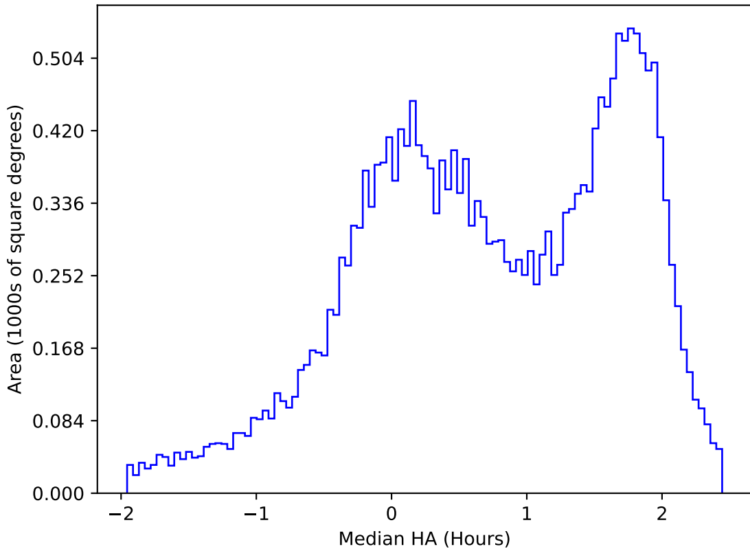
roll_pause_mjdp180_v3.4_10yrs All sky u band: Median HA
