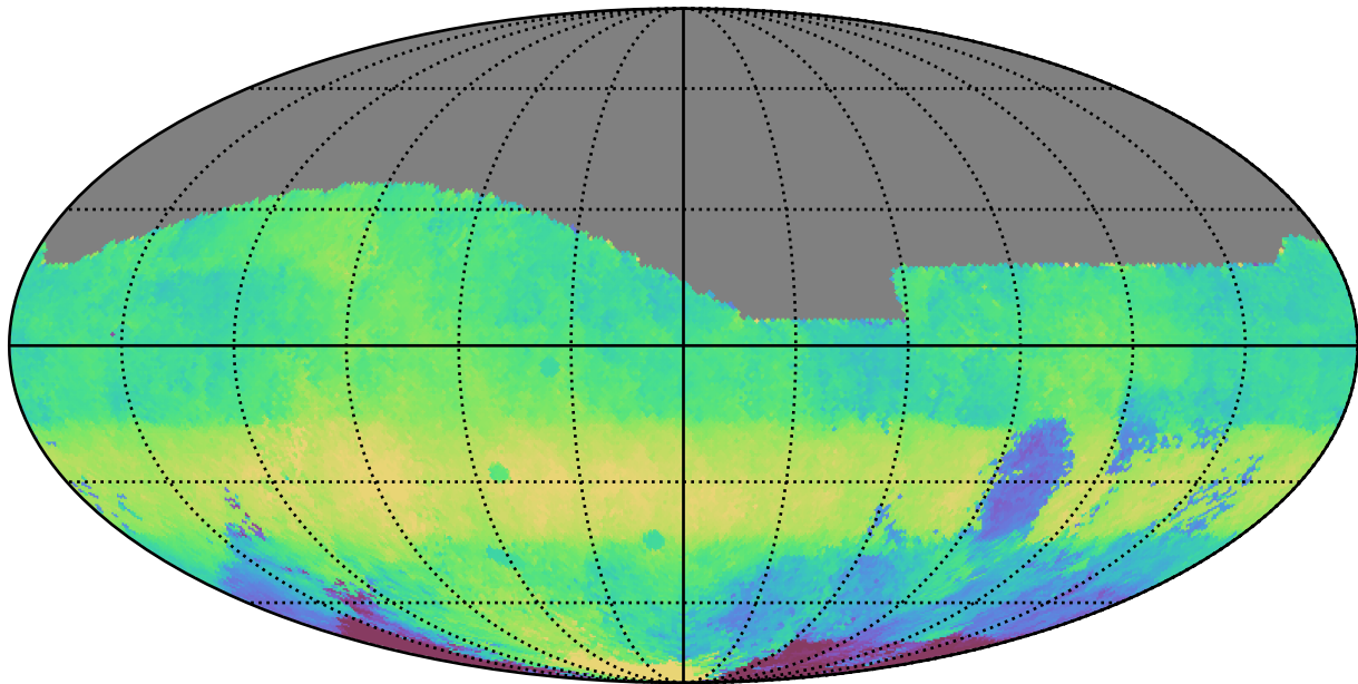
roll_pause_mjdp180_v3.4_10yrs All sky g band: Median HA
