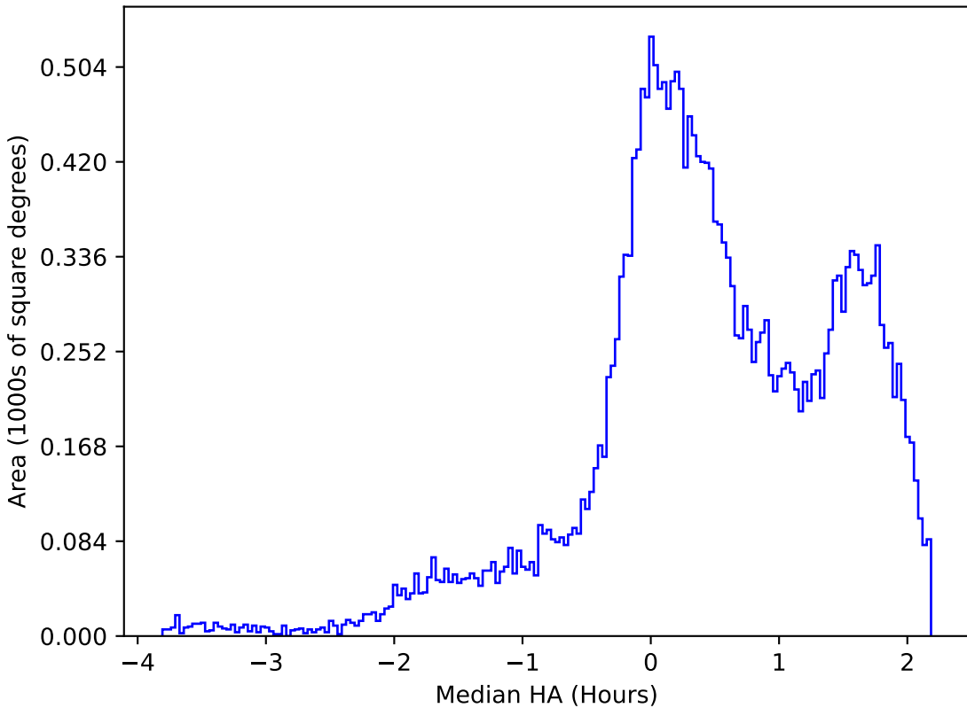
roll_pause_mjdp180_v3.4_10yrs All sky g band: Median HA
