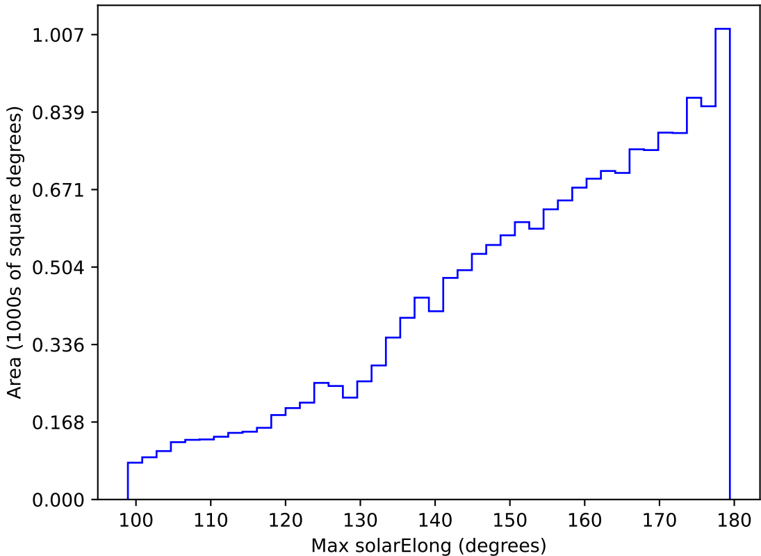
roll_pause_mjdp180_v3.4_10yrs WFD z band: Max solarElong
