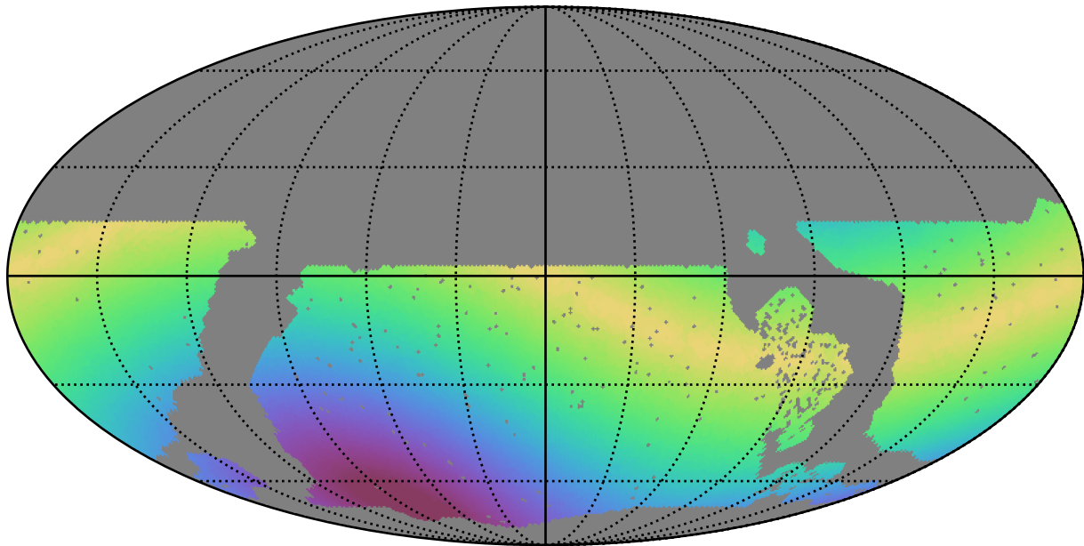
roll_pause_mjdp180_v3.4_10yrs WFD y band: Max solarElong
