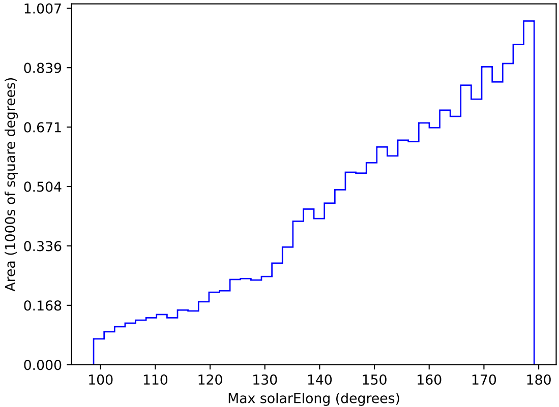
roll_pause_mjdp180_v3.4_10yrs WFD y band: Max solarElong
