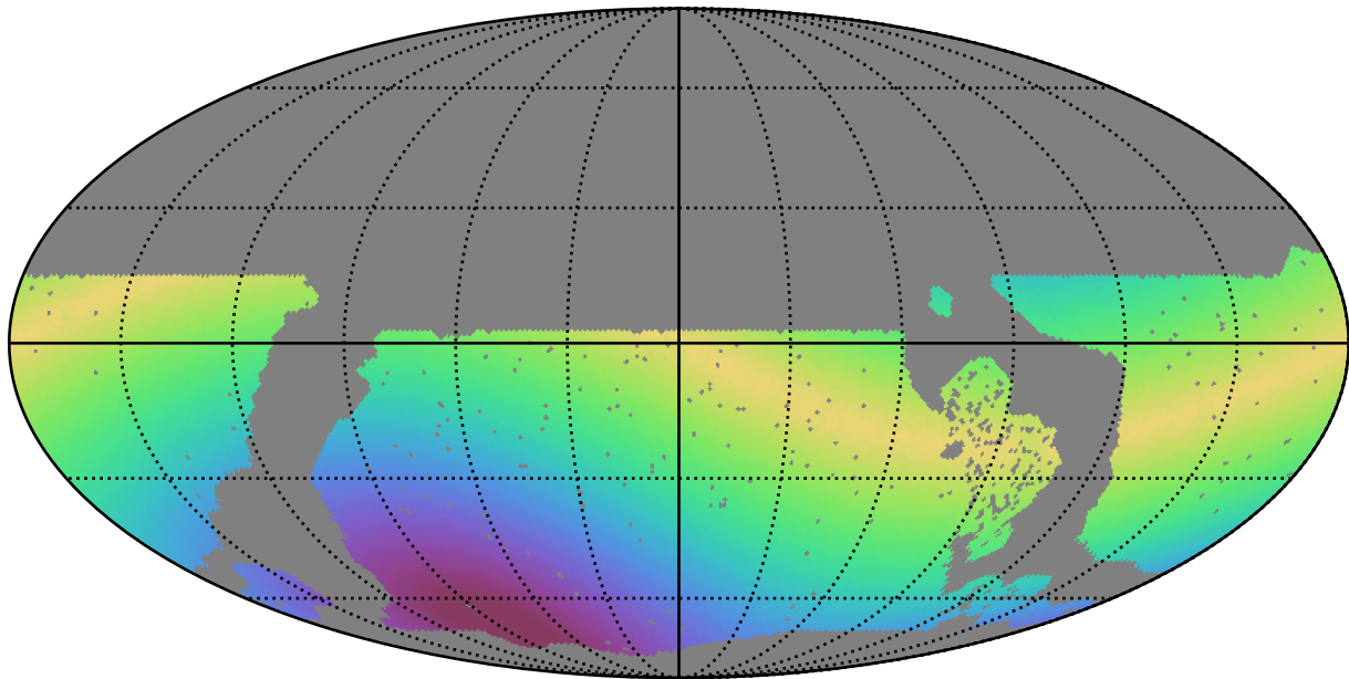
roll_pause_mjdp180_v3.4_10yrs WFD r band: Max solarElong
