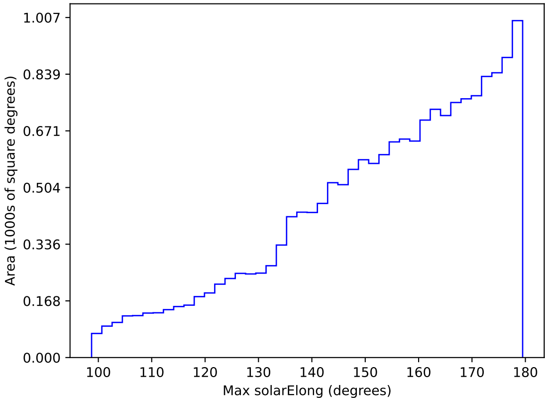
roll_pause_mjdp180_v3.4_10yrs WFD r band: Max solarElong
