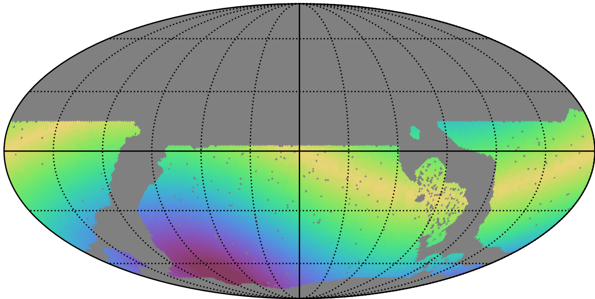
roll_pause_mjdp180_v3.4_10yrs WFD g band: Max solarElong
