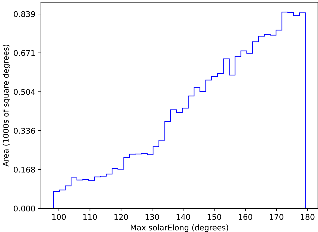
roll_pause_mjdp180_v3.4_10yrs WFD g band: Max solarElong
