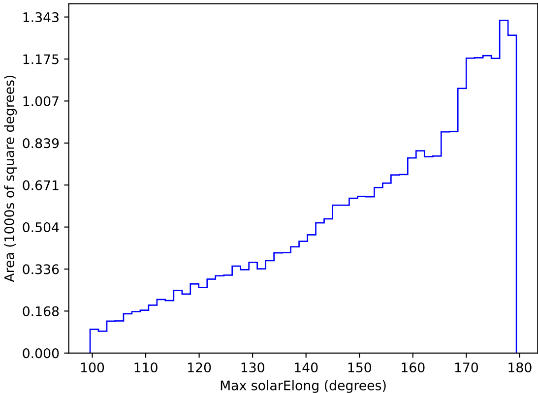
roll_pause_mjdp180_v3.4_10yrs All sky z band: Max solarElong
