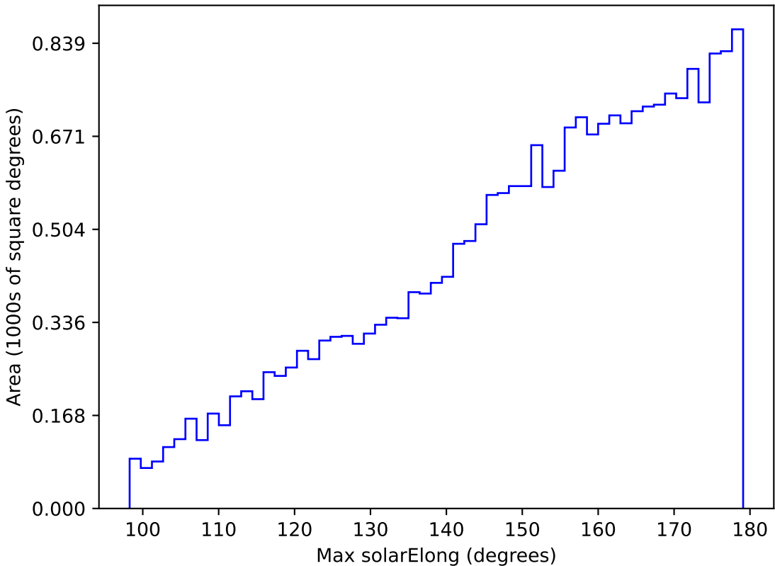
roll_pause_mjdp180_v3.4_10yrs All sky y band: Max solarElong
