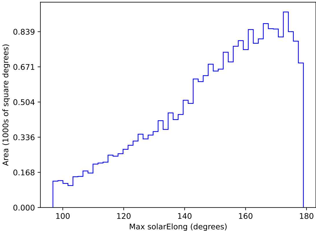
roll_pause_mjdp180_v3.4_10yrs All sky u band: Max solarElong
