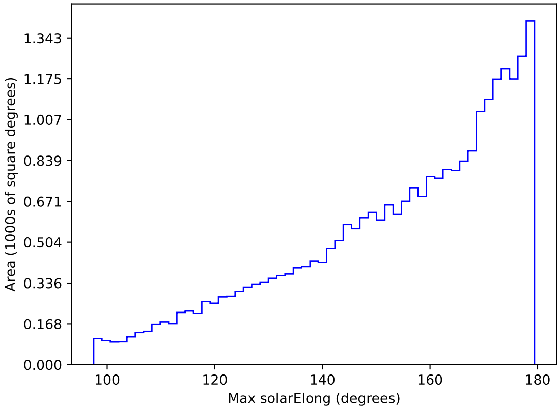
roll_pause_mjdp180_v3.4_10yrs All sky r band: Max solarElong
