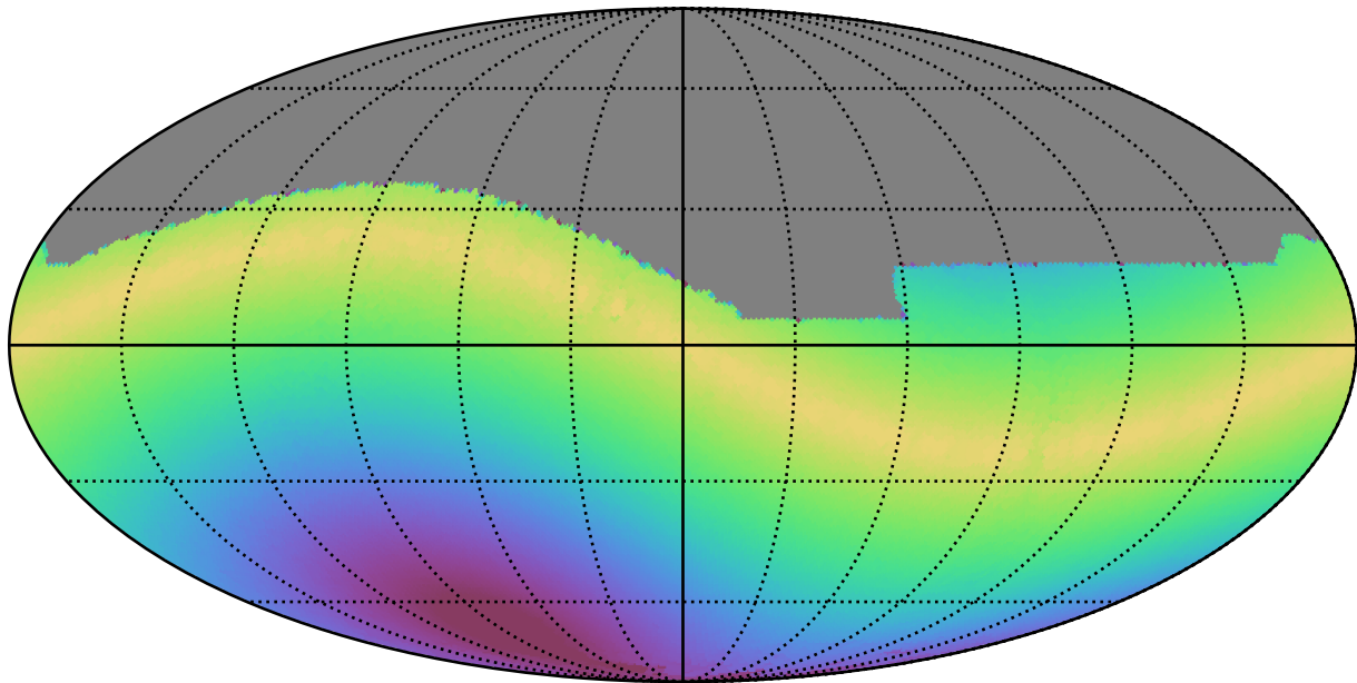
roll_pause_mjdp180_v3.4_10yrs All sky i band: Max solarElong
