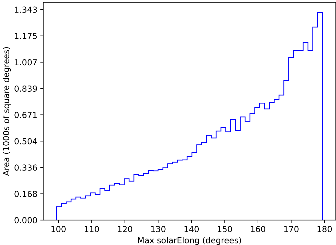
roll_pause_mjdp180_v3.4_10yrs All sky i band: Max solarElong
