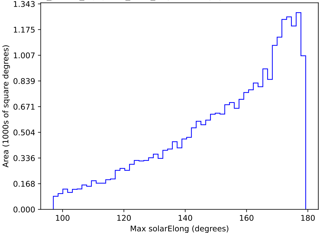
roll_pause_mjdp180_v3.4_10yrs All sky g band: Max solarElong
