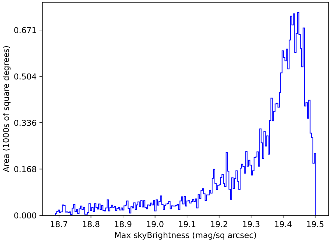
roll_pause_mjdp180_v3.4_10yrs Yr 1 z band: Max skyBrightness
