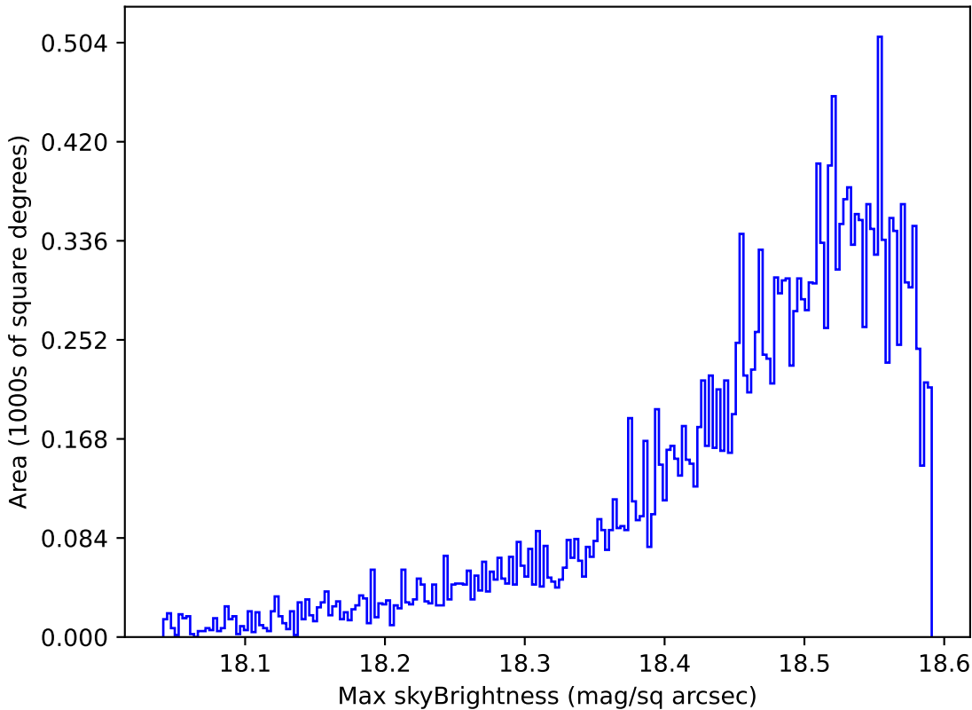
roll_pause_mjdp180_v3.4_10yrs Yr 1 y band: Max skyBrightness
