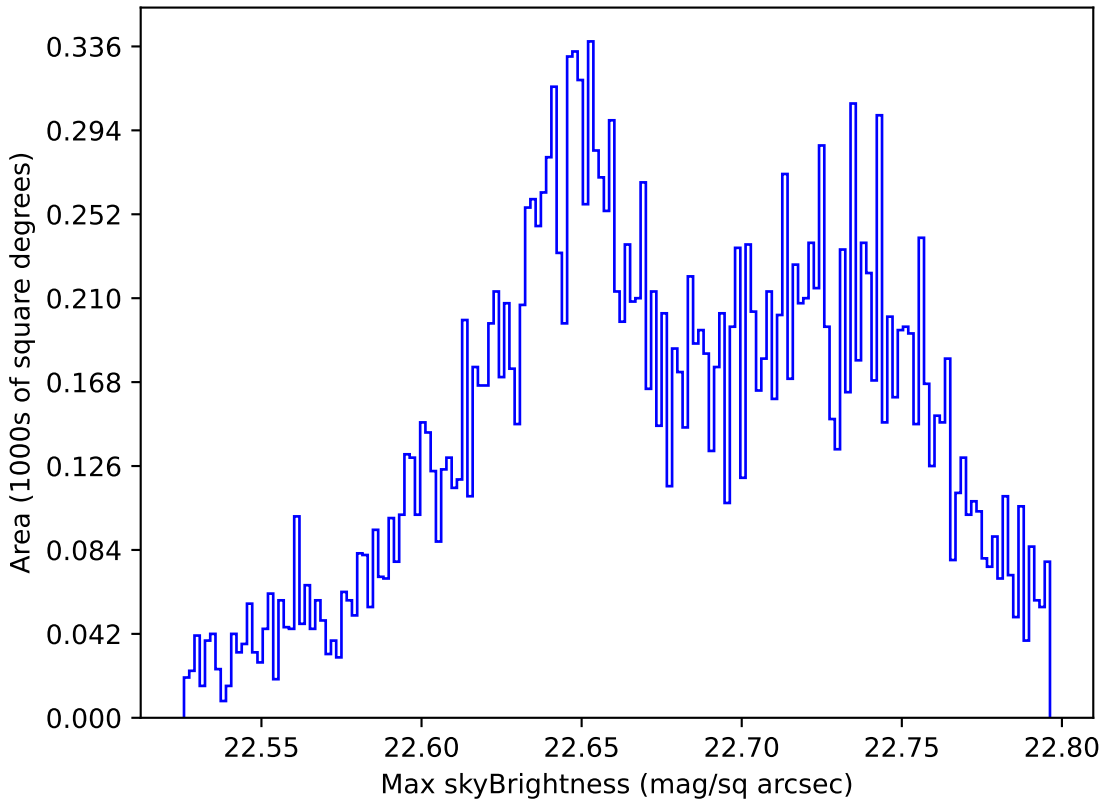
roll_pause_mjdp180_v3.4_10yrs Yr 1 u band: Max skyBrightness
