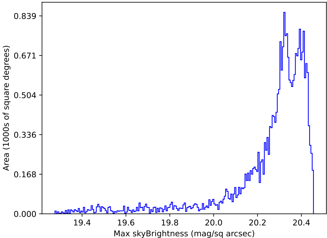
roll_pause_mjdp180_v3.4_10yrs Yr 1 i band: Max skyBrightness
