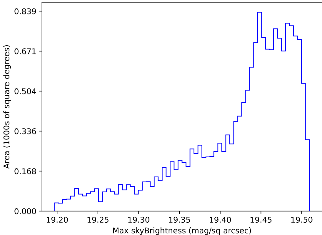
roll_pause_mjdp180_v3.4_10yrs WFD z band: Max skyBrightness
