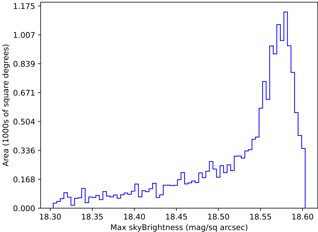
roll_pause_mjdp180_v3.4_10yrs WFD y band: Max skyBrightness
