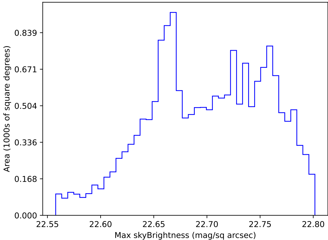
roll_pause_mjdp180_v3.4_10yrs WFD u band: Max skyBrightness
