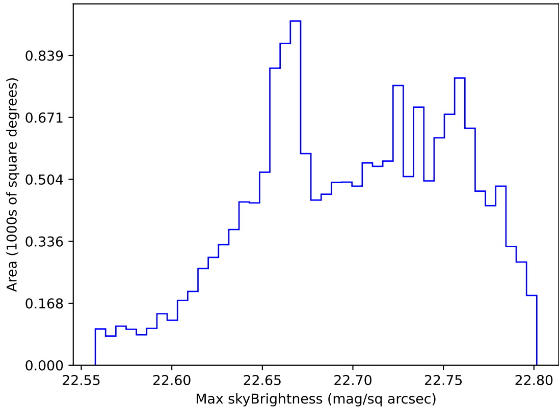
roll_pause_mjdp180_v3.4_10yrs WFD all bands: Max skyBrightness
