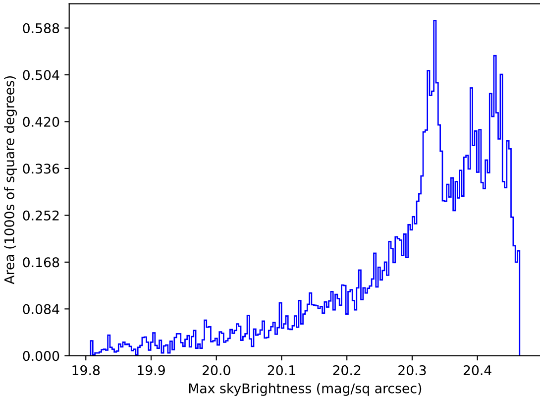
roll_pause_mjdp180_v3.4_10yrs All sky i band: Max skyBrightness
