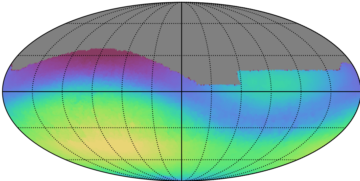
roll_pause_mjdp180_v3.4_10yrs All sky g band: Max skyBrightness
