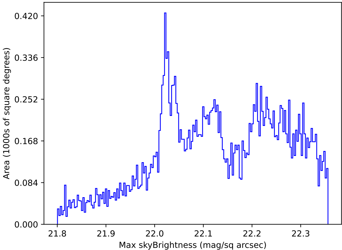
roll_pause_mjdp180_v3.4_10yrs All sky g band: Max skyBrightness
