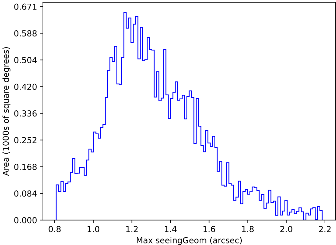
roll_pause_mjdp180_v3.4_10yrs Yr 1 z band: Max seeingGeom
