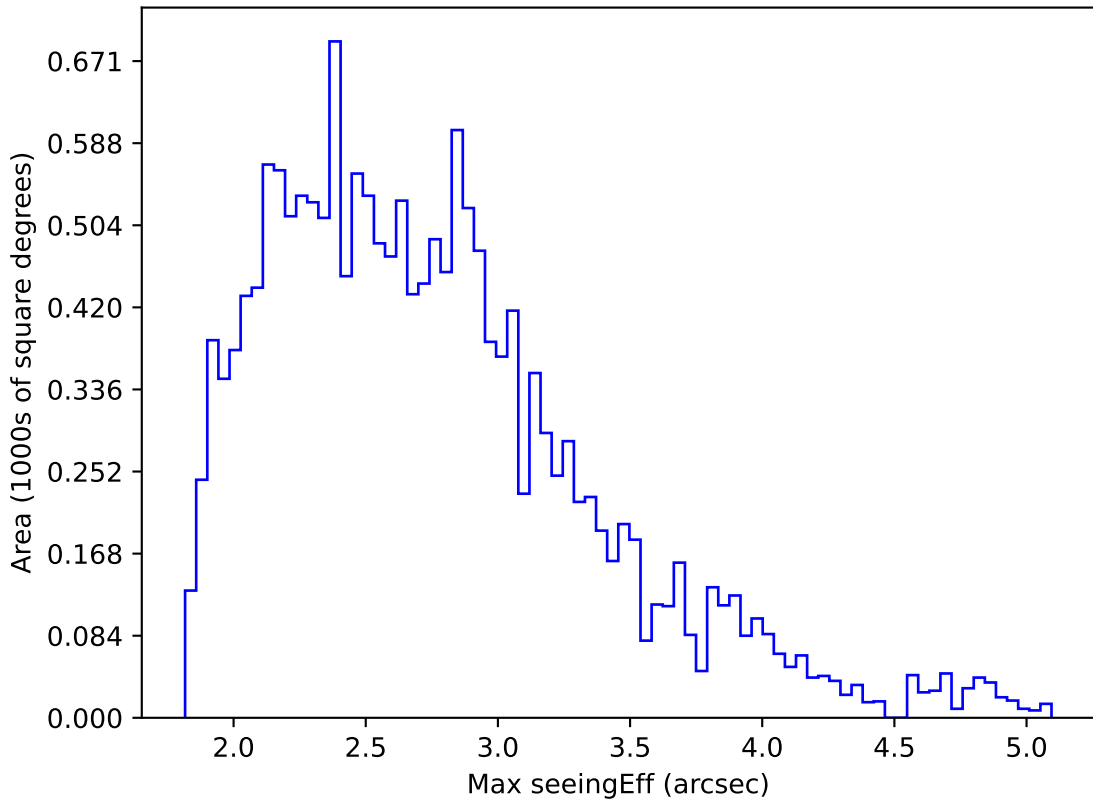
roll_pause_mjdp180_v3.4_10yrs WFD r band: Max seeingEff
