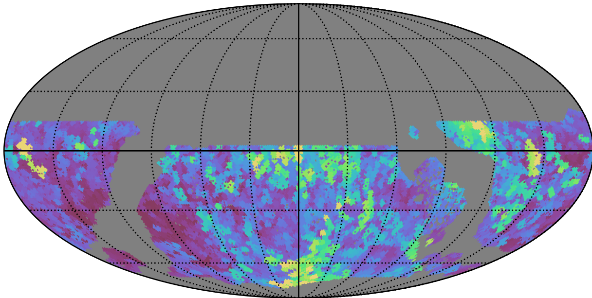
roll_pause_mjdp180_v3.4_10yrs WFD all bands: Max seeingEff
