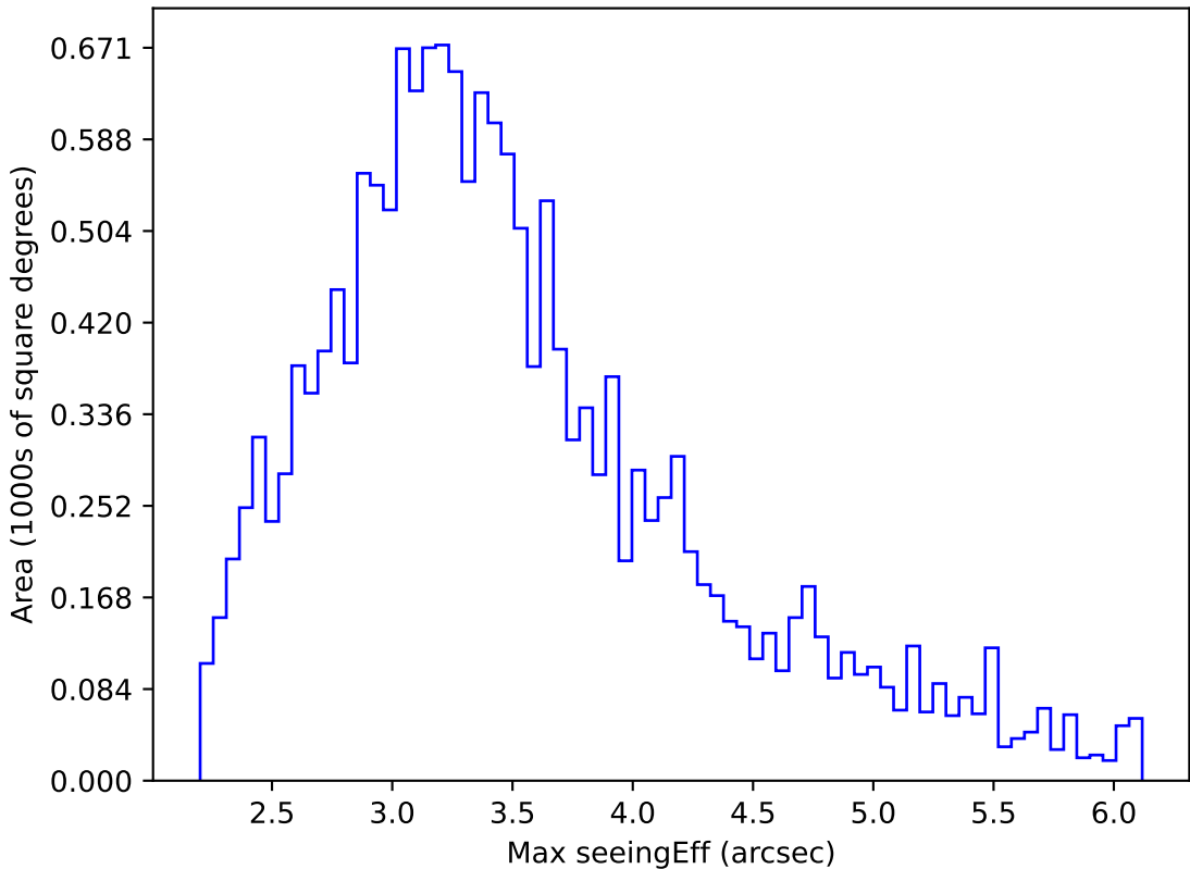
roll_pause_mjdp180_v3.4_10yrs WFD all bands: Max seeingEff
