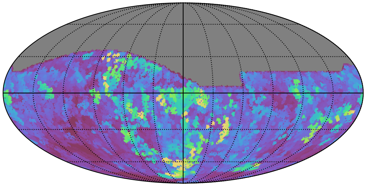
roll_pause_mjdp180_v3.4_10yrs All sky z band: Max seeingEff
