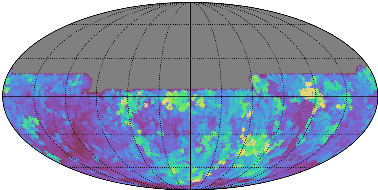
roll_pause_mjdp180_v3.4_10yrs All sky y band: Max seeingEff
