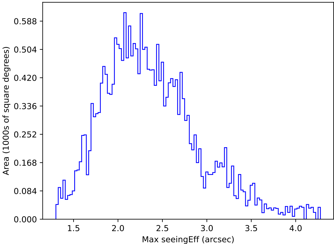
roll_pause_mjdp180_v3.4_10yrs All sky y band: Max seeingEff
