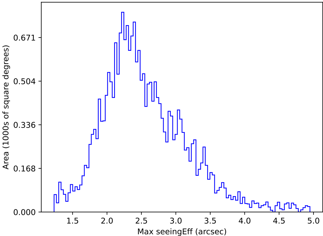
roll_pause_mjdp180_v3.4_10yrs All sky u band: Max seeingEff
