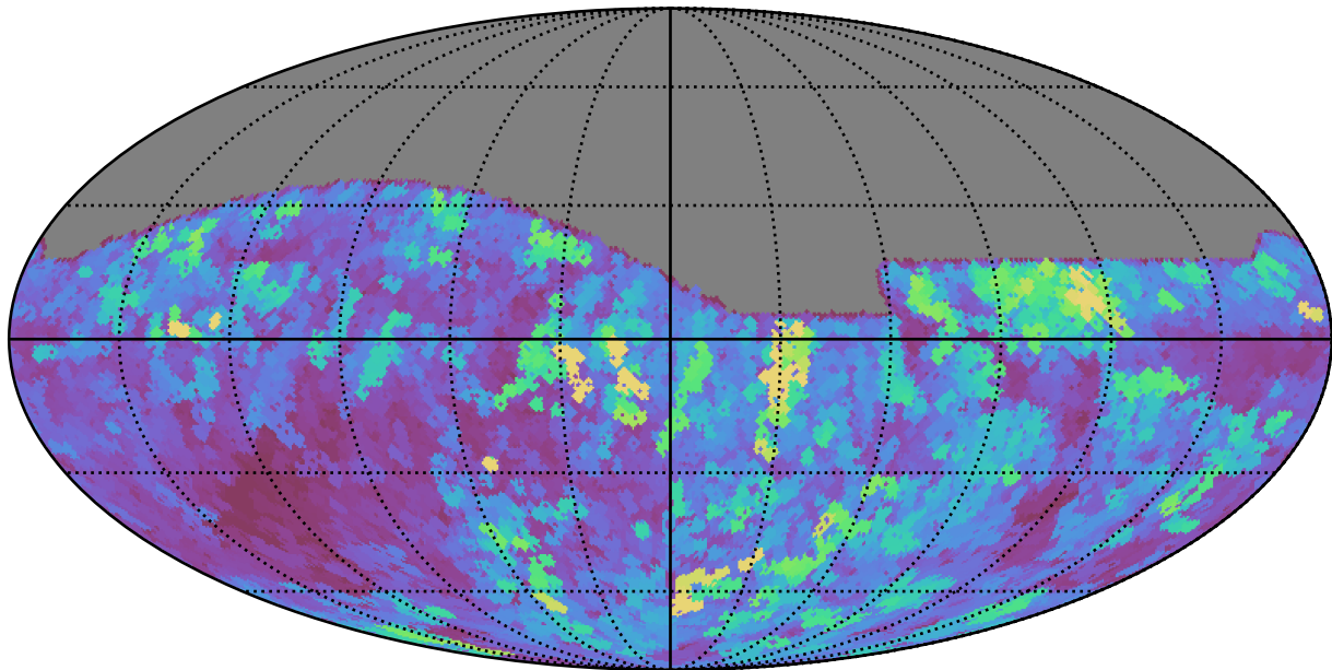
roll_pause_mjdp180_v3.4_10yrs All sky r band: Max seeingEff
